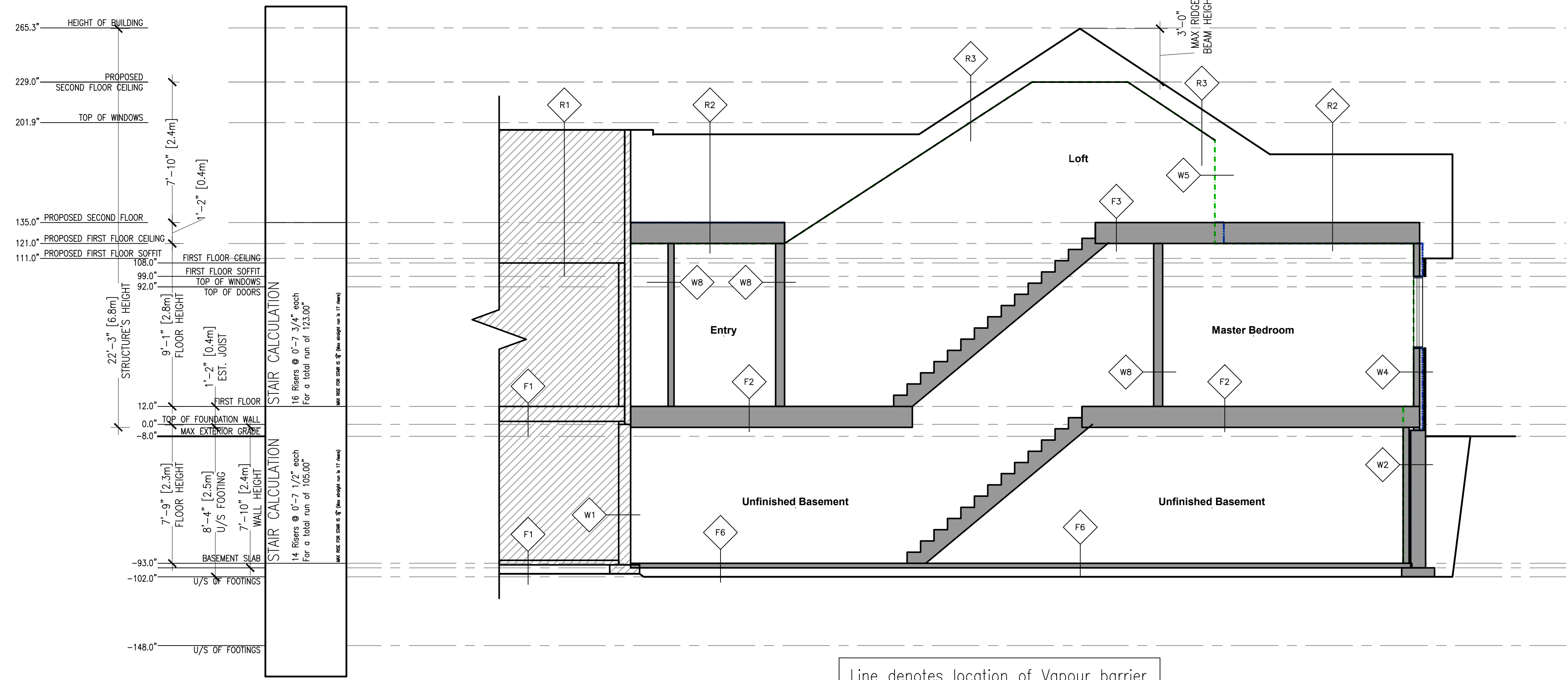
A Section 1 VO1 SCALE 1/4" = 1'-0"
